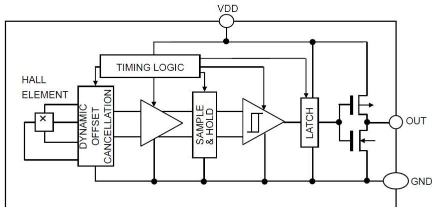
Figure 3, Block Diagram of AS1833A
