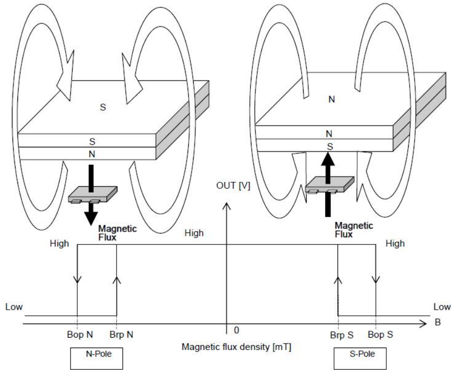
Fig 4, Magnetic Operation Characteristic of AS1833A
